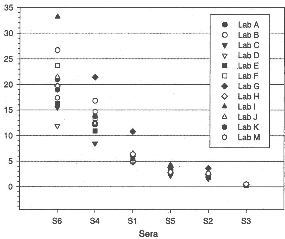
Figure 7 — Relative potencies for each of the sera as determined in the different laboratories (A-K and M). The y axis represents the relative potencies (mean of 3 calculations)
