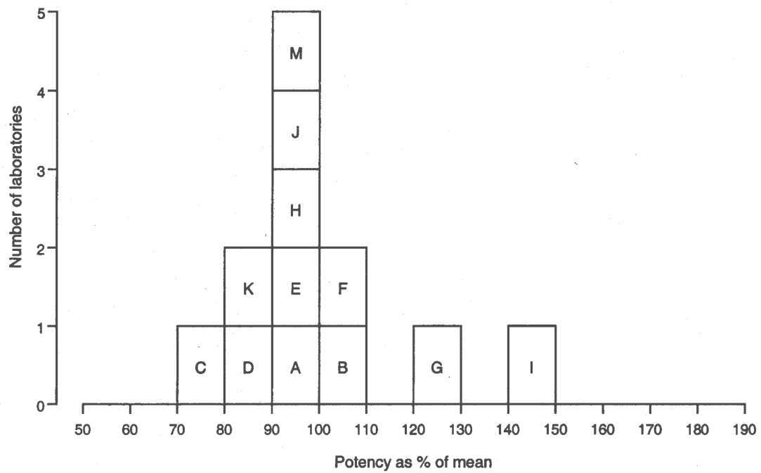
Figure 5 — Serum 5 potency as a percentage of the overall mean, for each laboratory
